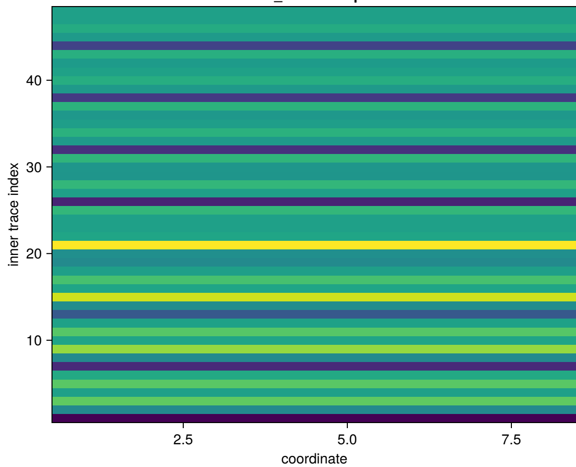
x_{\text{ref}} heatmap
